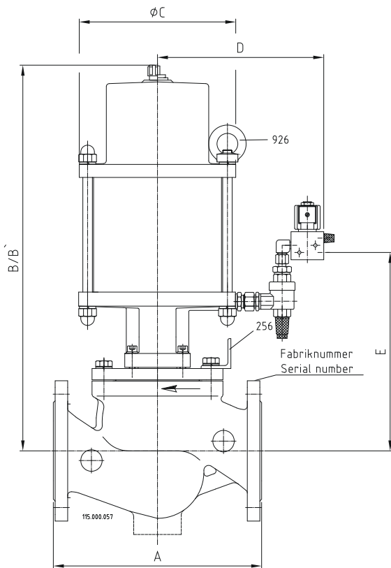
Abb.3 16/40-4 - AEPV...N(H)...
