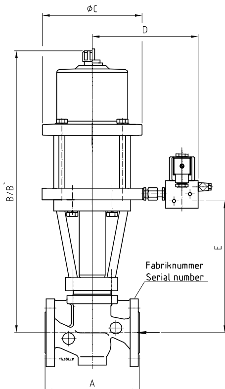
Abb.3 16/40-4 - AEPV...N(H)...
