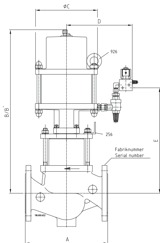
Abb.4 16/20/30-4 - AEPV...N(H)...
