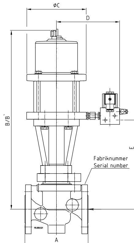
Abb.4 16/20/30-4 - AEPV...N(H)...
