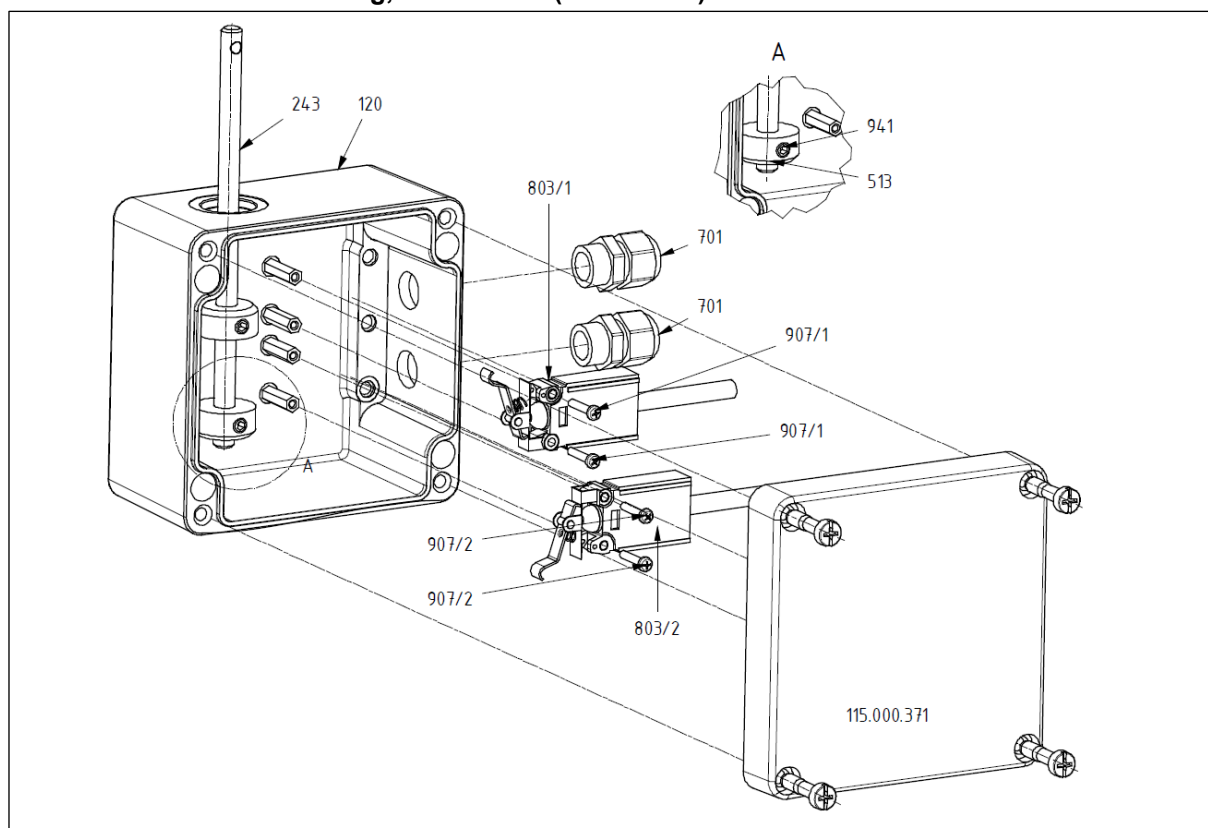
Part list (example of limit switch with cable gland)
