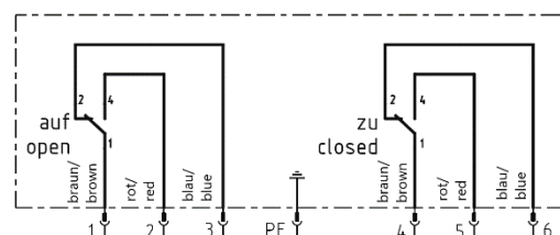
Wiring diagram
