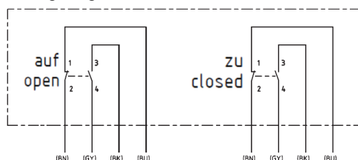
Wiring diagram
